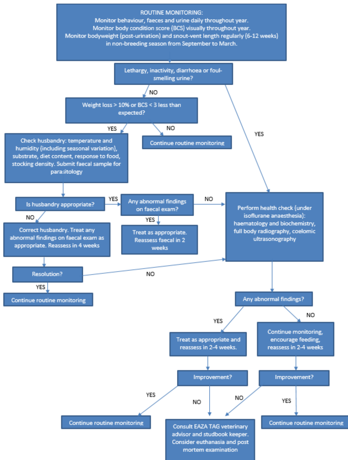
Figure 37. Decision making tree for management of body condition loss in Leptodactylus fallax .
